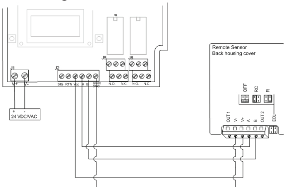
Figure 2. Connecting Main Sensor to Remote
